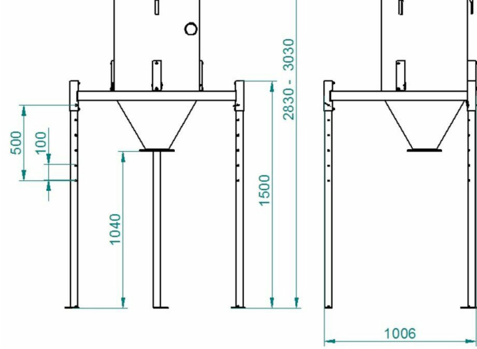
Dimensions with 1 500 mm legs
